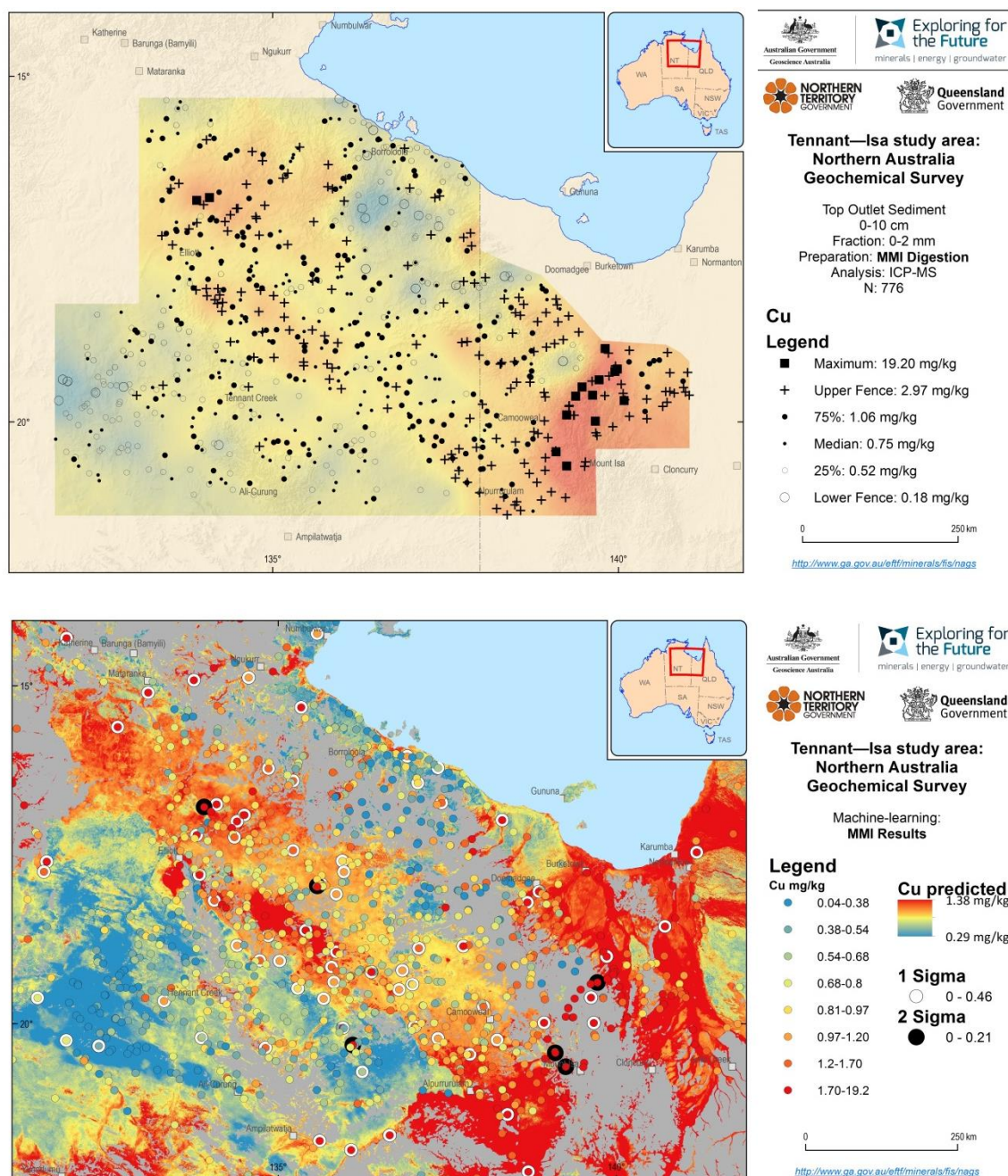
Figure A3.5.1. Map showing the distribution of copper in the Northern Australia Geochemical Survey (NAGS) samples over the Tennant Creek — Mt Isa study area. (A) Top map: The results of the MMI™ extraction (the sediment 0–2 mm fraction); (B) Bottom map: MMI™ Cu concentrations predicted by machine learning. Copper values above 1 and 2 \sigma values of the predictive model indicate sites where Cu concentration are clearly above the environmental background.
